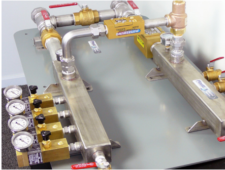
Special Pressure Balanced Manifold Assembly with Flow Regulators for Telescope Cooling Application
