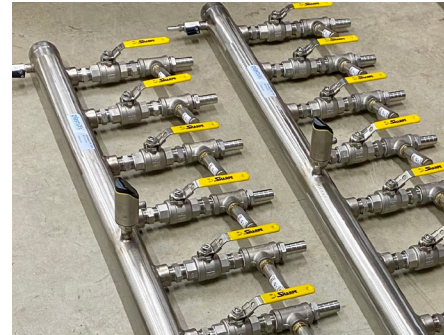
Large Supply Manifold Assemblies with Electronic Pressure Sensors, SS Valves, Hammer Arrestors and Drain Valves for Server Cooling Application
