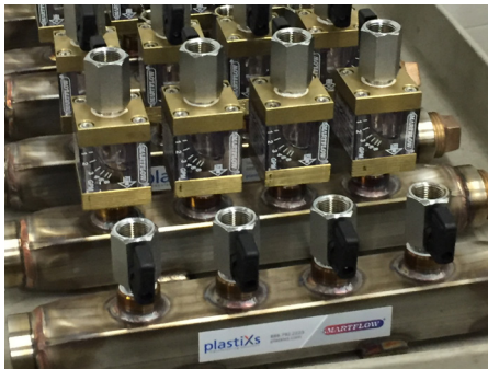
Supply and Return Manifold Pair Assemblies with Mini Ball Valves and Mechanical Flowmeters on the Return Side for Injection Molding Application
