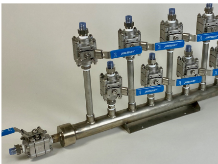
Custom Xtreme HiTemp Stainless Steel Manifold Assembly with End Port Connection and Staggered Valves with Special Center-to-Center Dimensions
