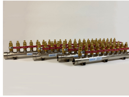
1 1/2" Special Compact Stainless Steel Manifold Assemblies with Full Port Brass Ball Valves and a Unique Pre-Threaded Mounting System
