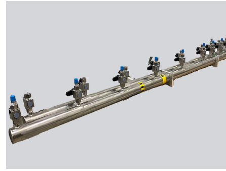
Large Custom Stainless Steel Manifold Assembly for Cooling Drive on Semiconductor Equipment
