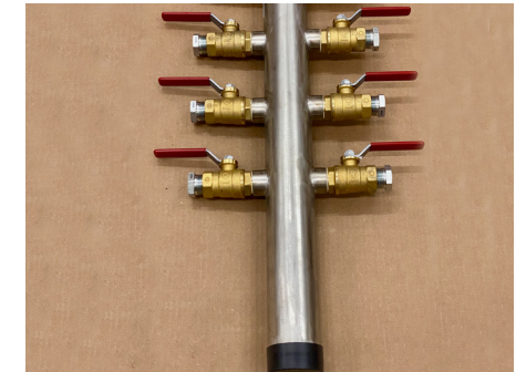
Custom Stainless Steel Manifold Assembly with 180° Ports Installed with Full Port Ball Valves for Welding Gases in an Automotive Frame Assembly Plant
