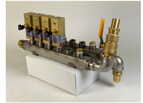
Custom Compact Stainless Steel Manifold Assembly with Flowmeters and Flow Regulators for Cooling Power Supplies
