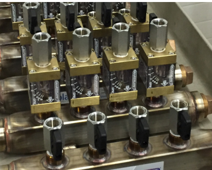
Supply and Return Manifold Pair Assemblies with Mini Ball Valves and Mechanical Flowmeters on the Return Side for Injection Molding Application
