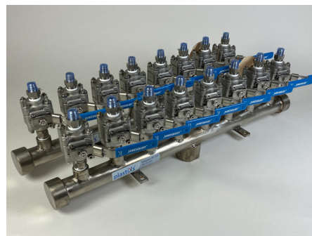
Xtreme HiTemp Stainless Steel Manifold Assemblies with Center Port Connection
